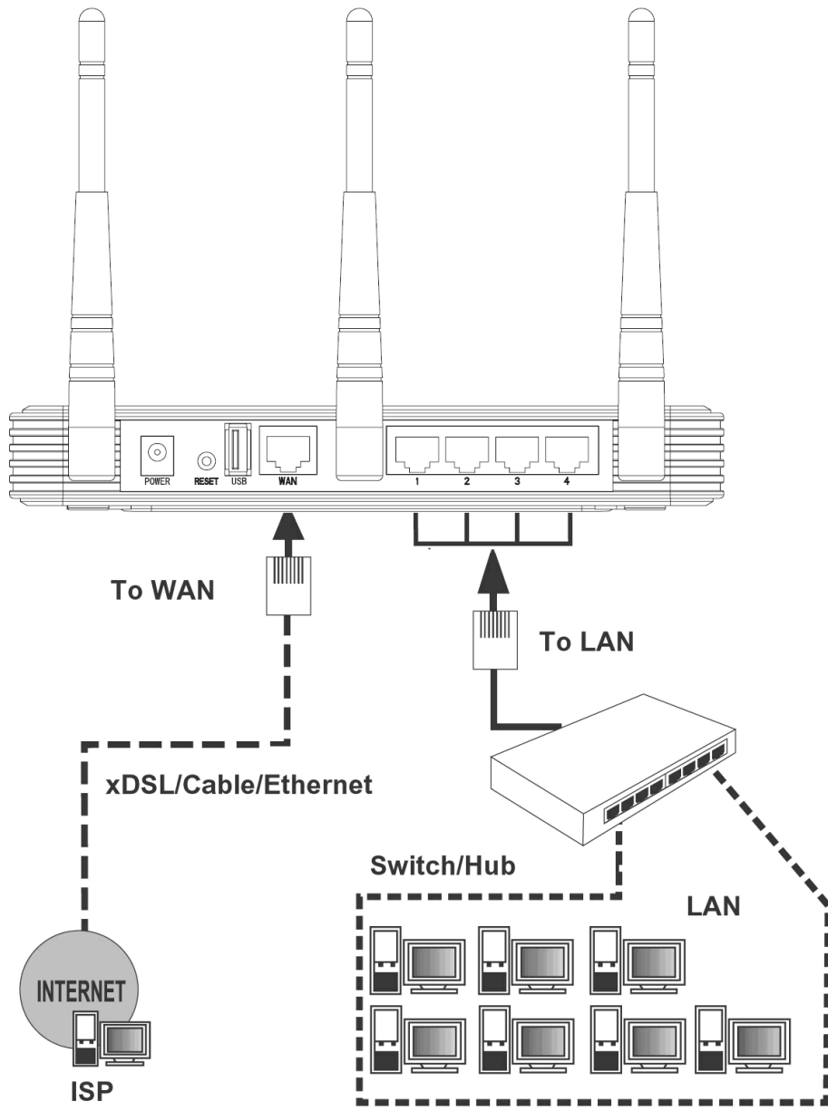
Figure 2-1 Hardware Installation of the TL-WR1043ND Wireless N Gigabit Router
