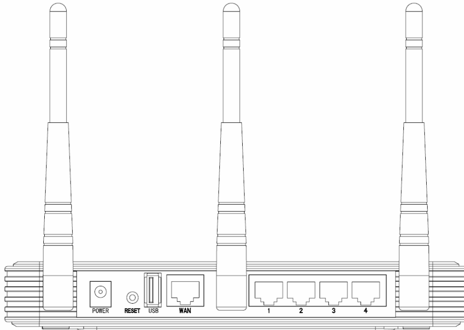
Figure 1-2 Rear Panel sketch
