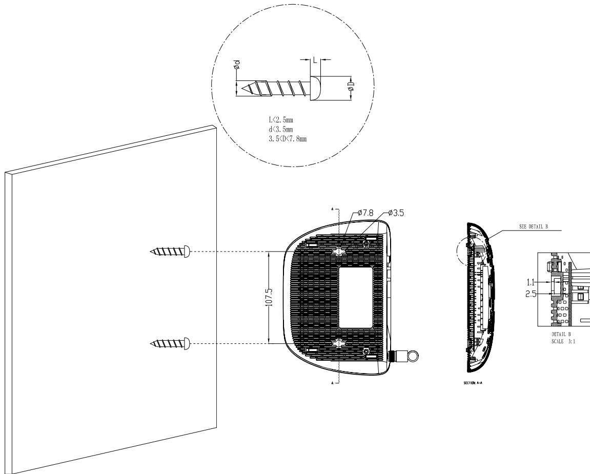
Figure 2-3 Wall-mount Install
